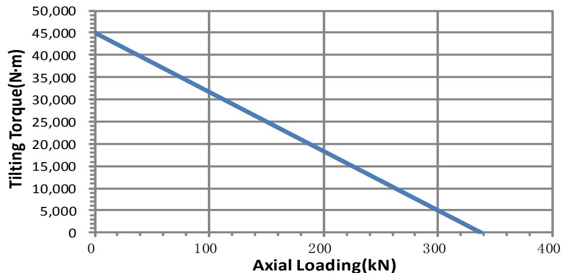
Tilting Torque VS Axial Loading
